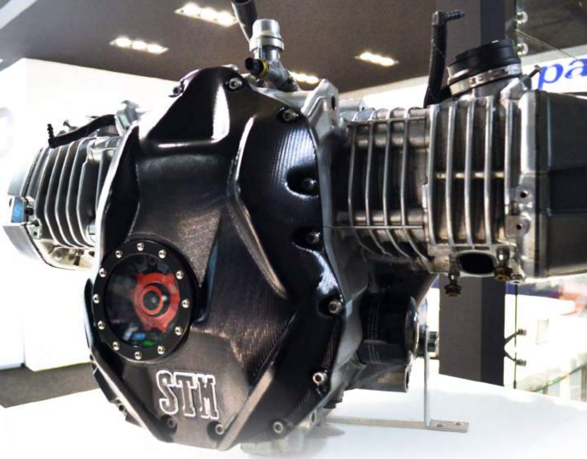
CARTER SCULTURATO E FRIZIONE BMW GS1200 SCULPTURED CARTER AND CLUTCH BMW GS1200
